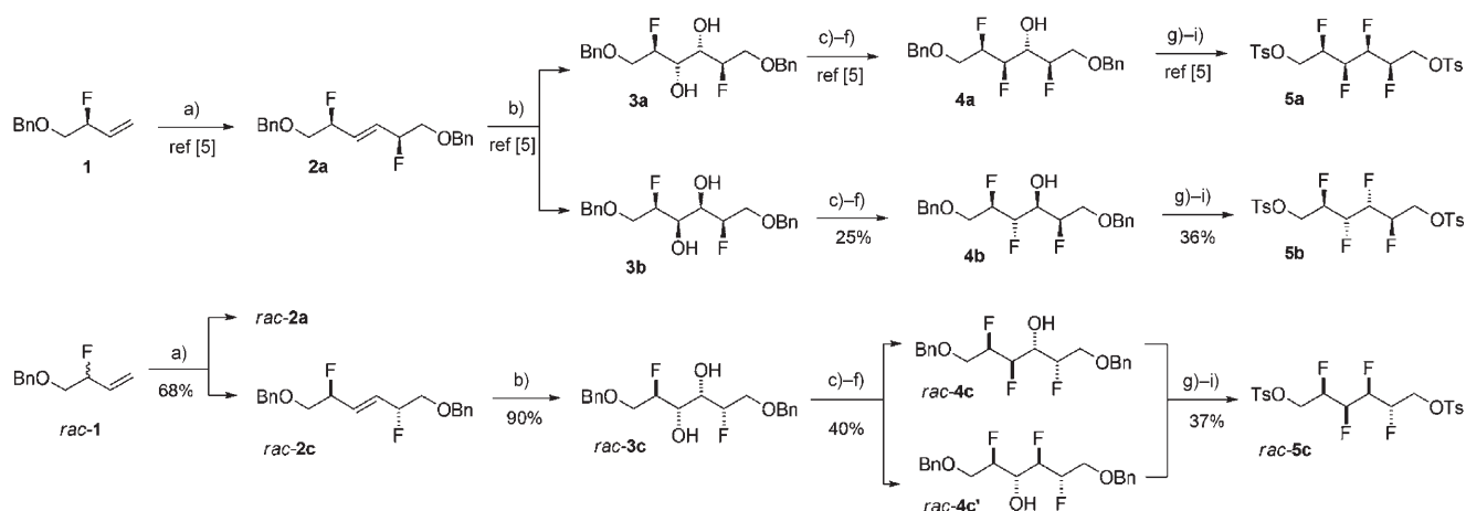
Scheme 1. Synthesis of 5a , [5] 5b and rac - 5c . Reagents and conditions: [6] a) Grubbs 2nd-generation catalyst, CH 2 Cl 2 , Δ; b) KMnO 4 , MgSO 4 , EtOH, CH 2 Cl 2 , H 2 O, 0°C; c) SOCl 2 , pyridine, CH 2 Cl 2 , room temperature; d) NaIO 4 , RuCl 3 , MeCN, H 2 O, room temperature; e) Bu 4 NF, MeCN, room temperature; f) H 2 SO 4 , H 2 O, tetrahydrofuran, RT; g) H 2 , Pd/C, MeOH, room temperature; h) TsCl, collidine, 50°C; i) (MeOCH 2 CH 2 ) 2 NSF 3 (Deoxo-Fluor), CH 2 Cl 2 , Δ.
